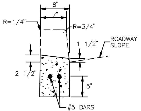
DEPRESSED CURB
