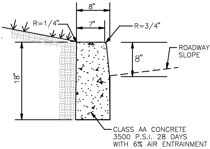
VERTICAL CURB
